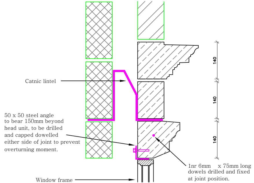
Typical Head Section Where Lower Head is in Multiple Pieces With No Central Support
