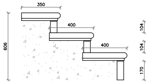
Typical Section
