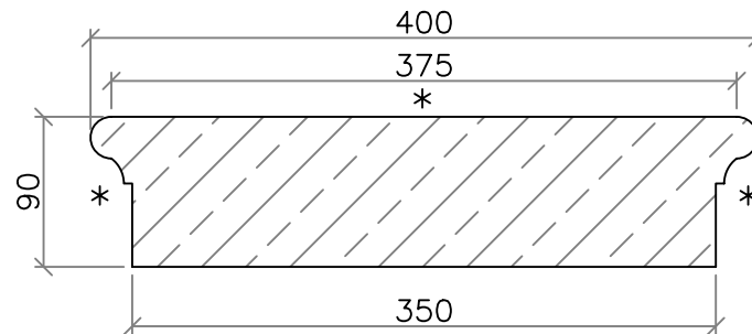
Typical Section
