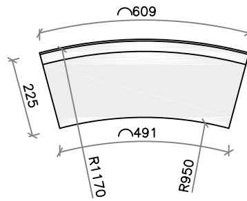
Plinth Detail
