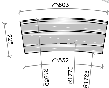
Kerb Detail
