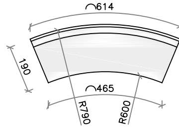
Plinth Detail
