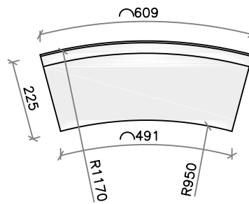
Plinth Detail
