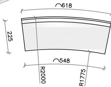
Plinth Detail
