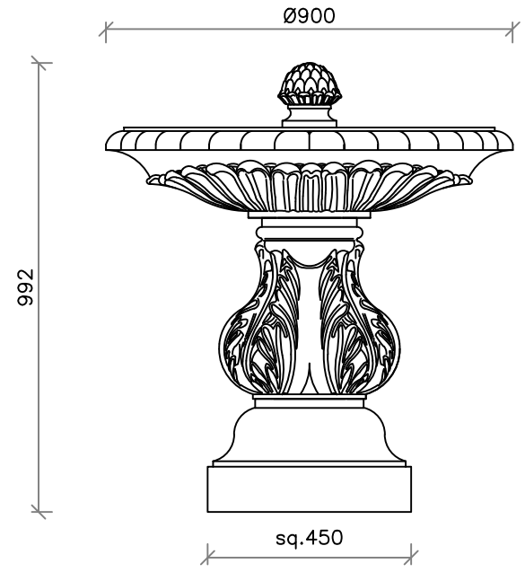
FT43 - Large Single Bowl
