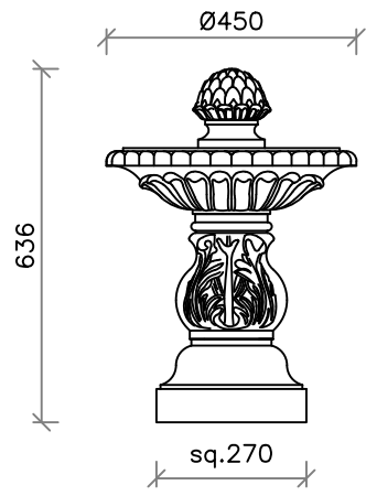
FT41 - Small Single Bowl
