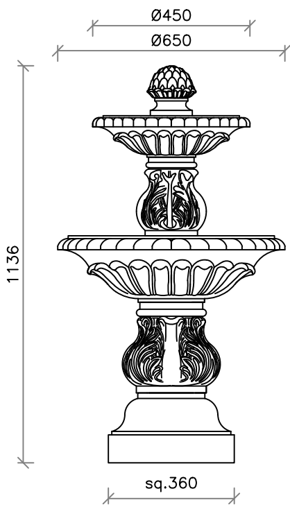
FT44 - Small Double Bowl
