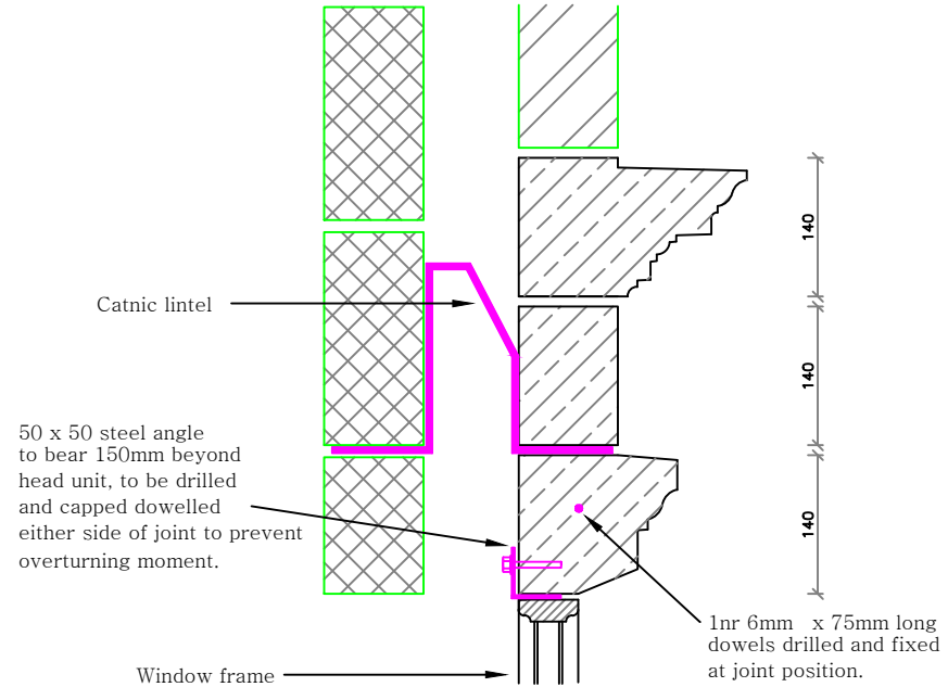
Typical Head Section Where Lower Head is in Multiple Pieces With No Central Support
