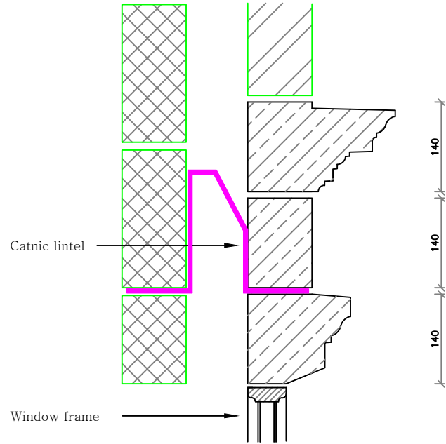
Typical Head Section Where Lower Head is in One Piece
