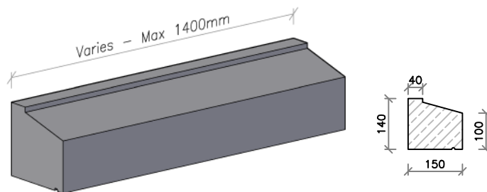
C2S Style (38kg/m)
