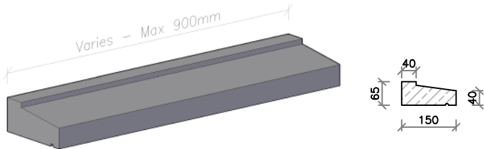
C3S Style (51kg/m)
