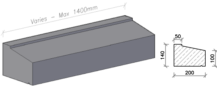
C3S Style (51kg/m)
