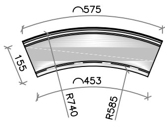
Kerb Detail
