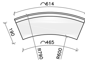
Plinth Detail
