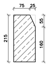
Section E-E
