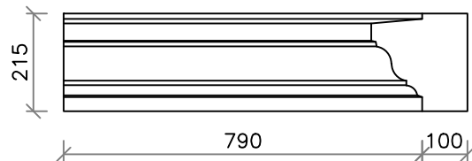
90° Internal Return - RH
