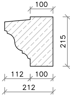
Typical X-Section
