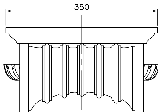
SIDE ELEVATION 1:5
