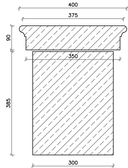
Typical Section
