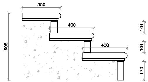
Typical Section
