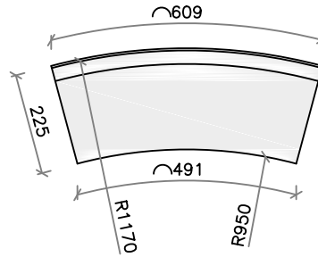
Plinth Detail
