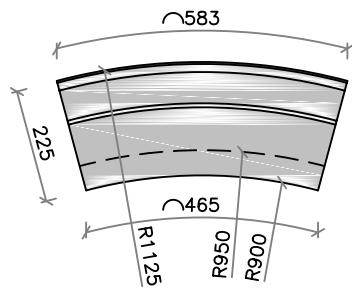
Kerb Detail
