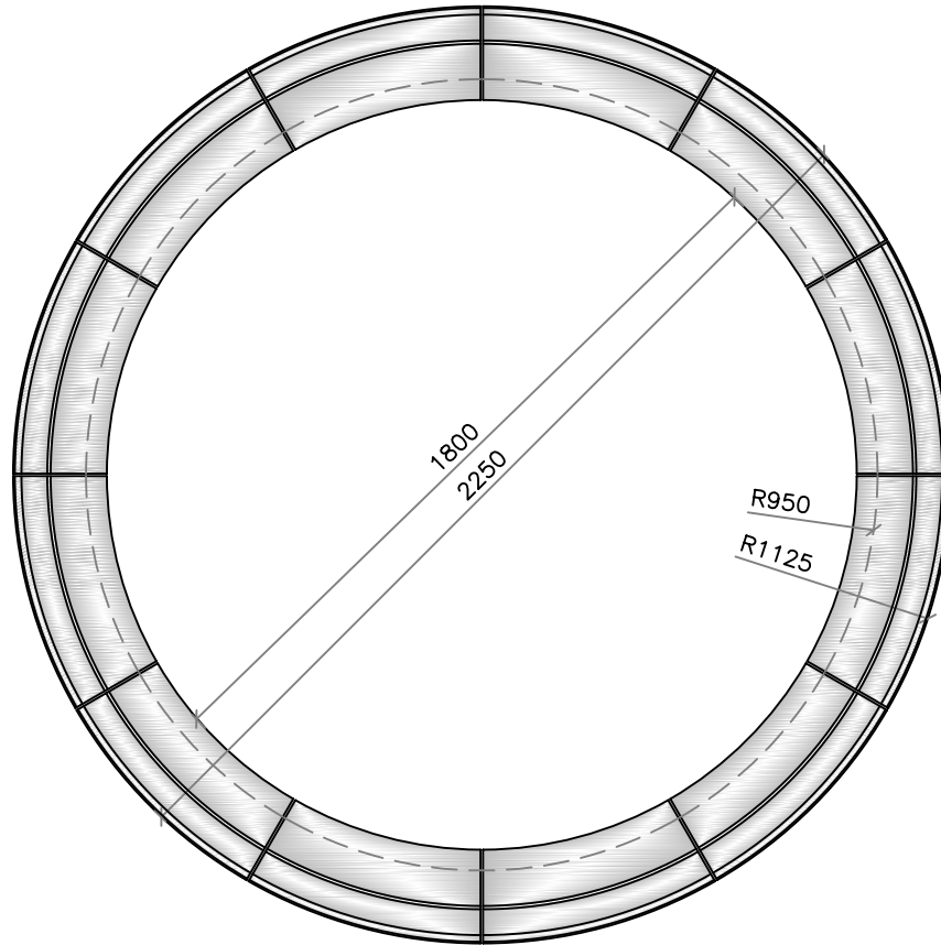
Plan View
