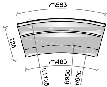
Kerb Detail
