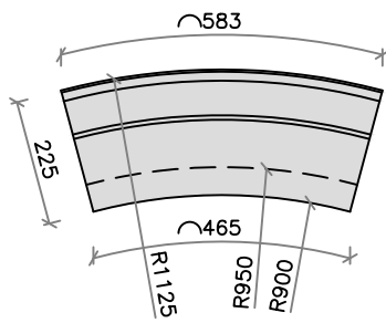
Kerb Detail
