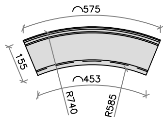
Kerb Detail
