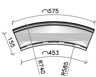
Kerb Detail
