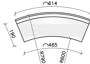
Plinth Detail
