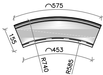
Kerb Detail
