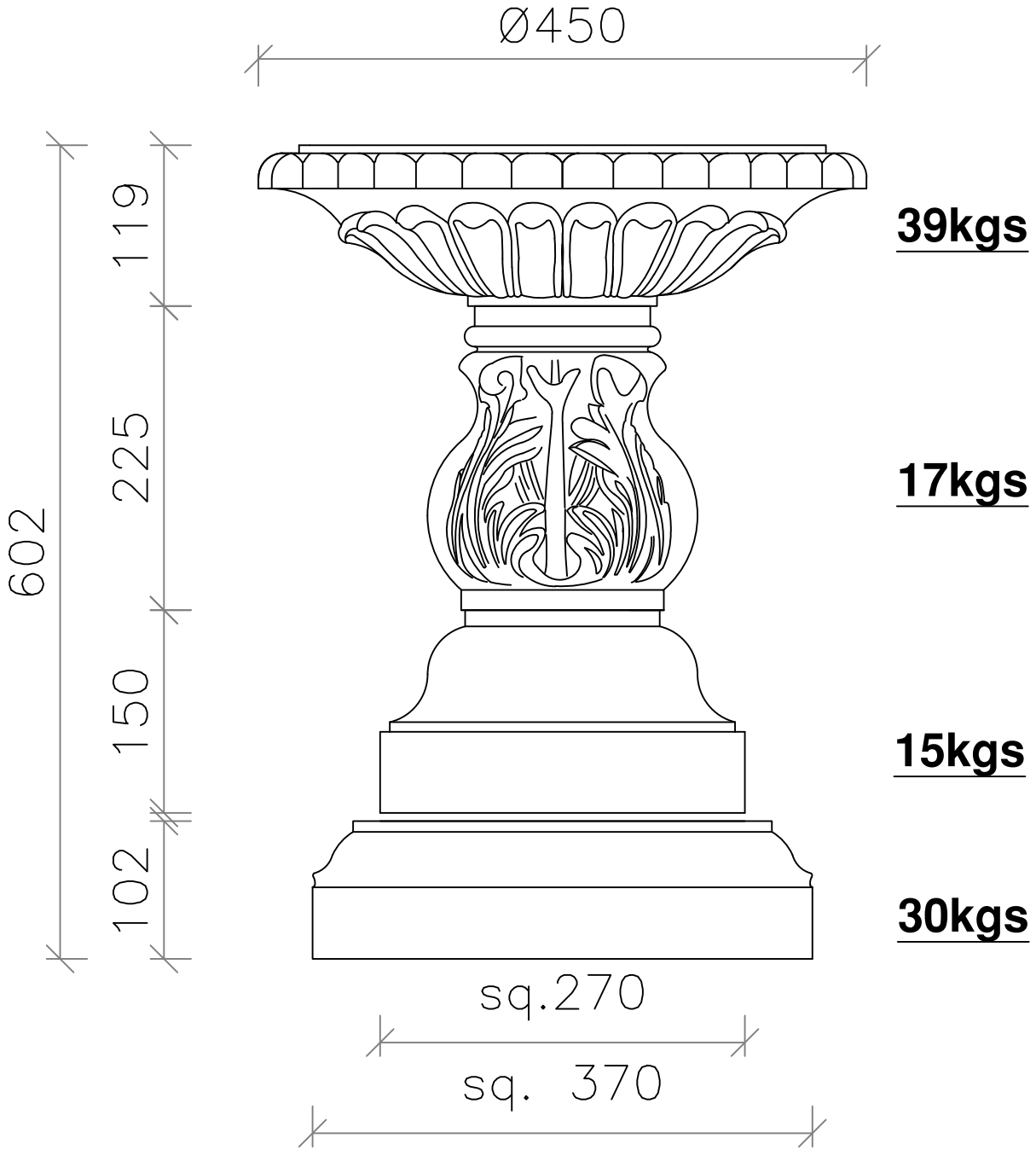
BB30 - Acanthus Bird Bath
