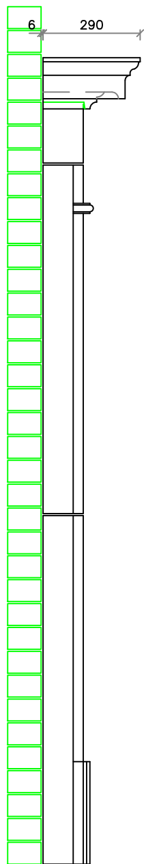
Side Elevation
