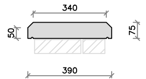
CS63 (36kg)
