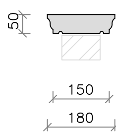
CS04B (10kg)
