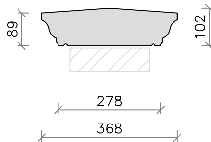
CS18 (41kg)
