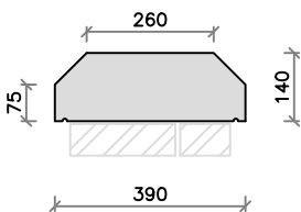
CS64 (63kg)
