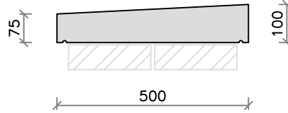
CS42 (55kg)
