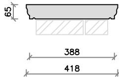
CS34B (33kg)
