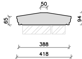
CS34C (45kg)
