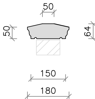
CS04C (12kg)
