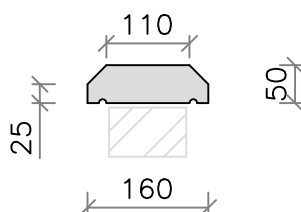
CS60 (9kg)
