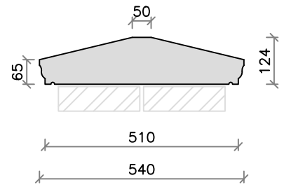
CS44C (65kg)
