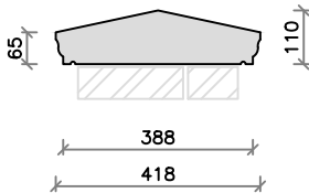
CS34 (45kg)
