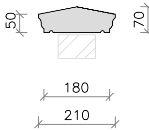
CS04A (15kg)
